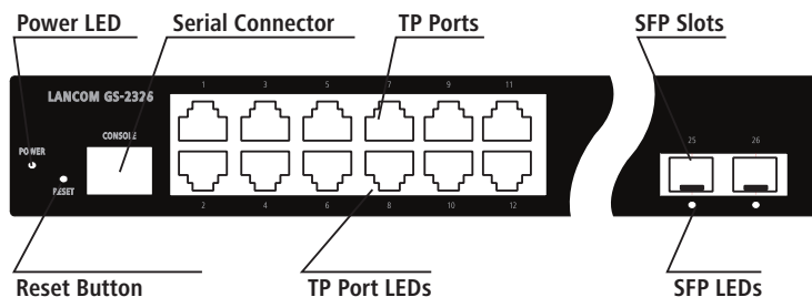
LANCOM GS-2326(P) front
