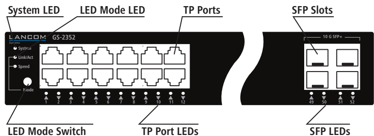
LANCOM GS-2352 front
